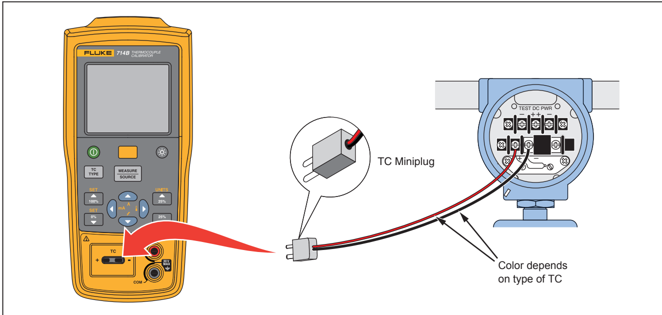
Figure 7. Connections for Simulating a Thermocouple
